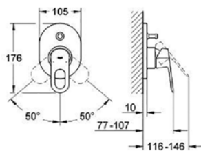
29 041 000 Shower/bath mixer with diverter
