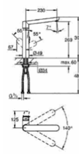
32 175 000 Sink mixer
