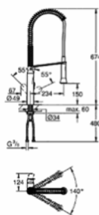
32 950 000 Professional sink mixer with Professional Spray with Pull-Out Dual Spray
