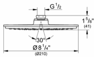
28 373 000 Overhead shower Rainshower 210
