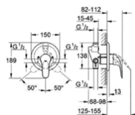
19 451 002 + 33 962 000 Shower/bath mixer
