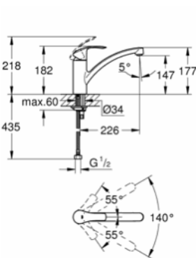
32 534 002 Sink mixer
