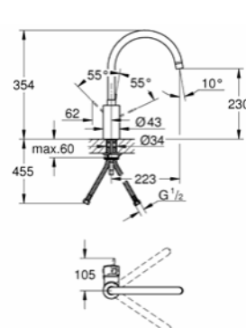
31 188 000 Sink mixer C-spout with Swivel Stop
