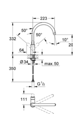
31 450 000 BauEdge Kitchen sink mixer
