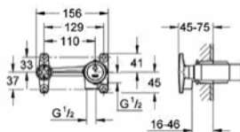
32 635 000 Wall mounted basin mixer set concealed body
