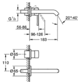
19 408 001 + 32 635 000 Wall mounted basin mixer set
