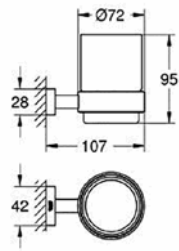
40 755 001 Glass tumbler holder
