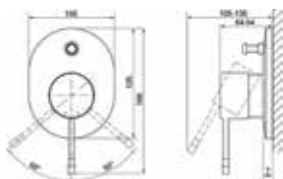
19 285 001SM + 33 961 000 Shower/bath mixer with diverter (Exclusive to ANZ)
