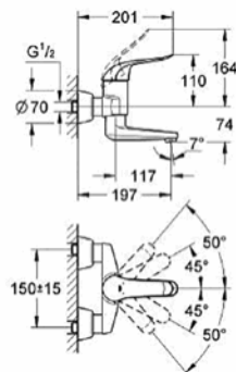
32 767 000 Euroeco Special Single-lever basin mixer, 1/2"
