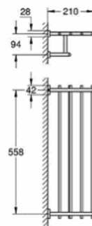
40 512 001 Multi-towel rack 558mm
