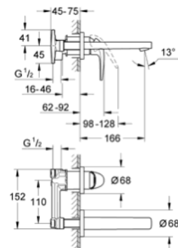
20 288 000 Wall basin mixer set
