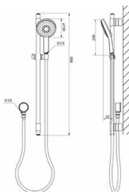
124 577 Shower rail set Power&Soul® Cosmopolitan 130
