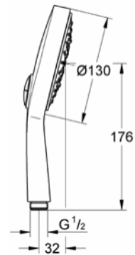
27 664 000 Hand shower 130
