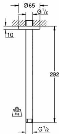
28 497 000 Ceiling shower arm metal length 292mm
