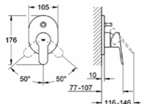
29 039 000 Shower/bath mixer with diverter
