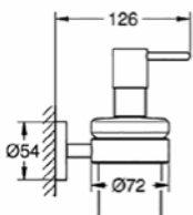
40 448 001 Soap dispenser with holder
