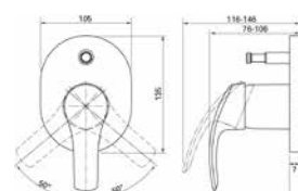
19 450 002SM + 33 961 000 Shower/bath mixer with diverter (Exclusive to ANZ)
