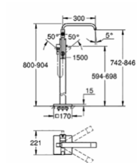
32 754 001 + 45 984 001 Bath/shower mixer floor mounted
