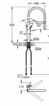
30 294 000 Professional sink mixer
