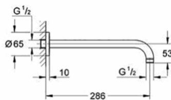
28 576 000 Shower arm metal projection 2 86mm
