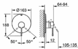
19 286 001 + 33 962 000 Shower/bath mixer
