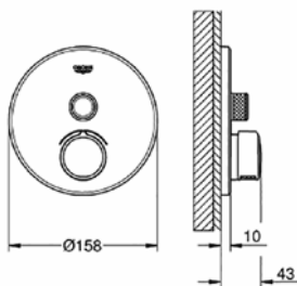
29 144 000 SmartControl mixer with 1 valve
