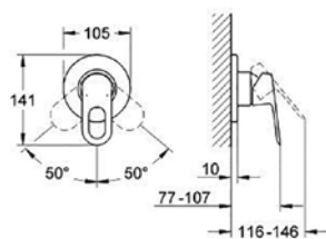
29 042 000 Shower/bath mixer
