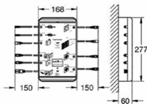
36 397 000 Base unit box 2.0 Bluetooth 26 374 000 Base unit box 4.0 Bluetooth
