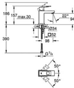
23 132 000 S-Size Basin mixer
