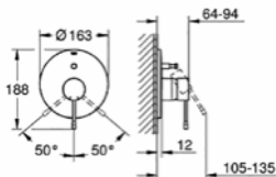
19 285 001 + 33 961 000 Shower/bath mixer with diverter
