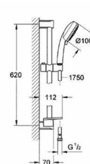
27 576 001 New Tempesta Cosmopolitan 100 Shower set with hand shower 3-spray
