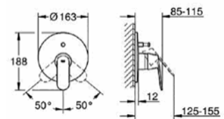
19 382 000 + 33 961 000 Shower/bath mixer with diverter
