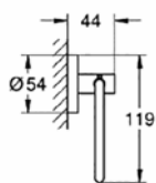
40 689 001 Toilet roll holder without cover
