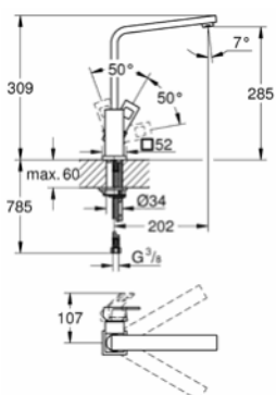
31 255 000 Single lever mixer with Swivel Spout
