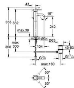
32 760 000 L-Size Basin mixer for free standing basin
