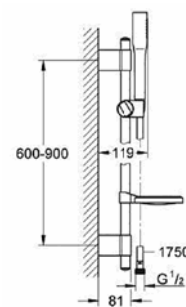
27 368 000 Shower set with hand shower Euphoria Cosmopolitan Stick
