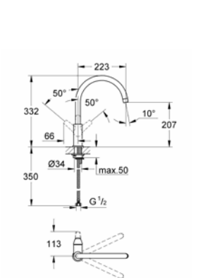
31 230 000 BauFlow Kitchen sink mixer
