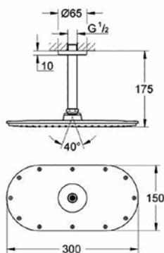
26 059 000 Veris 300 Head shower set length 142mm
