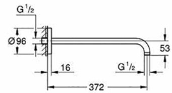
28 982 000 Shower arm metal projection 3 78mm
