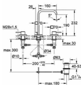
20 188 000 L-Size 3-hole basin mixer
