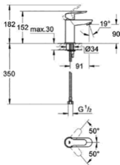
23 176 000 Basin mixer
