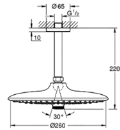
26 460 000 Euphoria 260 Headshower with wall arm
