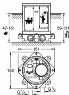
29 086 000 Floormounted bath/shower mixer concealed body
