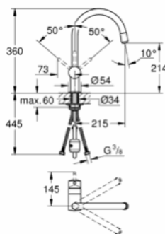
32 918 000 Minta sink mixer with Pull-Out Spray
