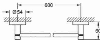
40 366 001 Towel rail 600mm
