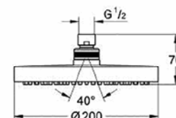
27 541 000 New Tempesta Cosmopolitan 200 Head shower
