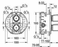
35 500 000 Thermostatic mixer concealed body
