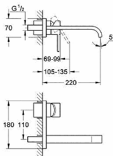
19 386 000 + 33 769 000 Wall mounted basin mixer set
