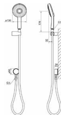
124 571 Hand shower set Power&Soul® Cosmopolitan 130
