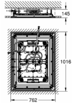
26 373 001 F-Series 40'' AquaSymphony
