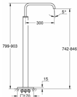
13 218 000 Bath spout
