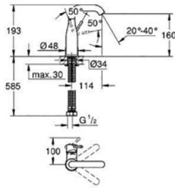
23 488 001 Gooseneck basin mixer
