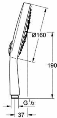
27 668 000 Power&Soul Cosmopolitan Hand shower 160
