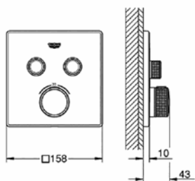
29 124 000 Grohtherm SmartControl thermostat for concealed installation with 2 valves
