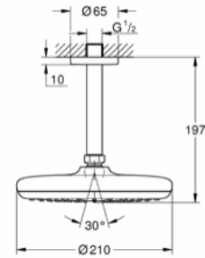
26 414 000 New Tempesta Cosmopolitan 210 Head shower with wall arm
