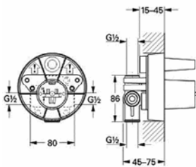
33 962 000 Shower/bath mixer concealed body
