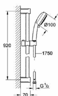
27 790 001 New Tempesta Cosmopolitan 100 Shower set with hand shower 4-spray rail 900mm
