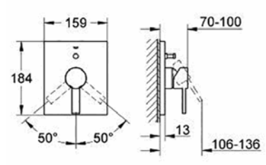
19 315 000SM Shower/bath mixer with diverter
