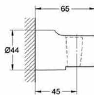
28 622 000 Relexa Wall hand shower holder non-adjustable
