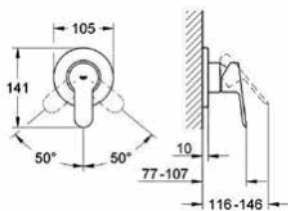
29 040 000 Shower/bath mixer
