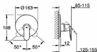
19 383 000 + 33 962 000 Shower/bath mixer
