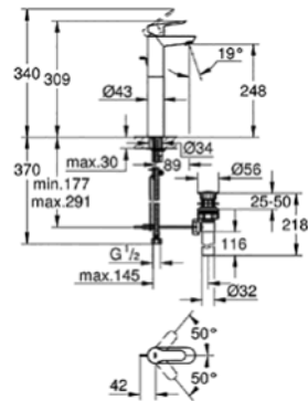
32 860 000 XL-Size Basin mixer
