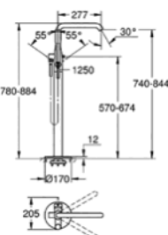
23 491 001 + 45 984 001 Floormounted bath/shower mixer
