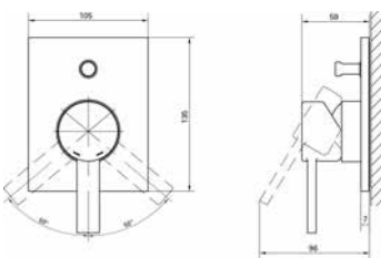
19 315 000 Shower/bath mixer with diverter (Exclusive to ANZ)
