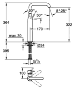
32 901 001 XL-Size Basin mixer
