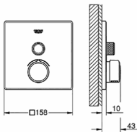
29 147 000 SmartControl mixer with 1 valve
