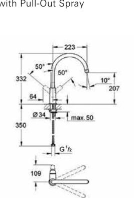
31 231 000 BauCurve Kitchen sink mixer
