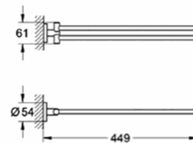
40 371 001 Double towel bar
