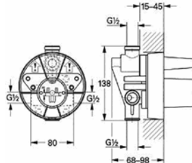
33 961 000 Shower/bath mixer with diverter concealed body
