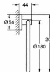
40 365 001 Towel ring
