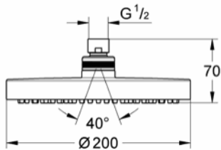
27 541 000 Overhead shower Tempesta 200
