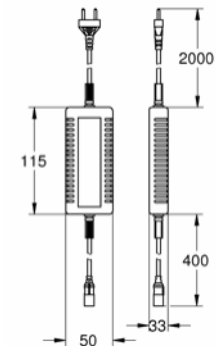
47 949 000 Power supply unit base box CN
