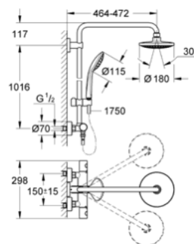
27 296 001 Euphoria 180 Shower System with Thermostat
