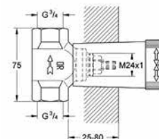
29 802 000 Concealed valve
