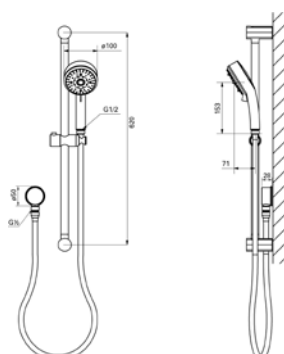
124 576 Shower rail set New Tempesta Cosmopolitan System 200
