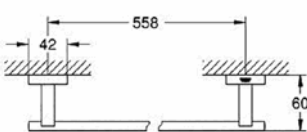
40 509 001 Towel rail 600mm
