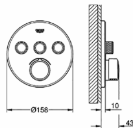
29 146 000 SmartControl mixer with 3 valves
