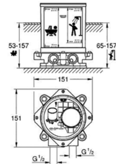
45 984 001 Floormounted bath/shower mixer concealed body
