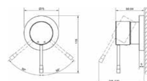
19 286 001SM + 33 962 000 Shower/bath mixer (Exclusive to ANZ)
