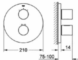
19 468 000 Grohtherm 3000 Cosmopolitan Thermostatic bath/shower mixer with integrated 2-way diverter
