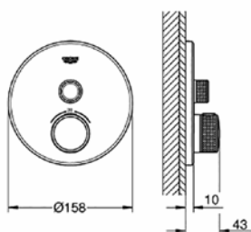
29 118 000 Grohtherm SmartControl thermostat for concealed installation with 1 valve
