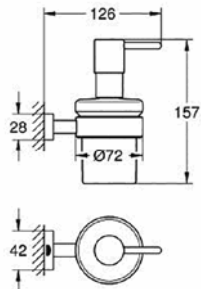
40 756 001 Soap dispenser with holder
