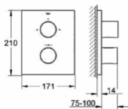
27 618 000 Grohtherm F Thermostatic Module with 2-way AquaDimmer
