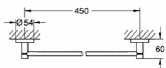
40 688 001 Towel rail 450mm
