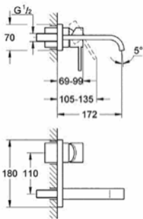
19 309 000 + 33 769 000 Wall mounted basin mixer set
