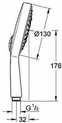
27 664 000 Power&Soul Cosmopolitan Hand shower 130
