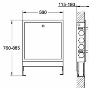
36 367 000 Rough-in set base unit box
