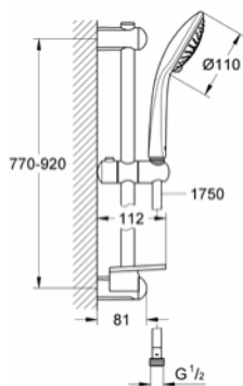
27 227 001 Euphoria 110 Champagne Shower rail set
