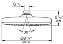
26 409 000 New Tempesta Cosmopolitan 210 Head shower
