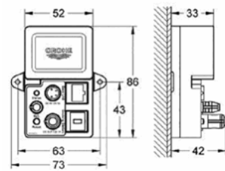
36 371 000 Bluetooth unit
