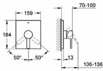
19 317 000SM Shower/bath mixer
