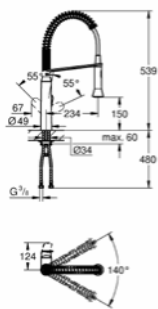
31 379 000 Professional sink mixer with Professional Spray with Pull-Out Dual Spray
