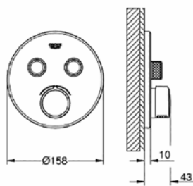
29 145 000 SmartControl mixer with 2 valves
