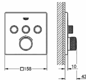
29 126 000 Grohtherm SmartControl thermostat for concealed installation with 3 valves
