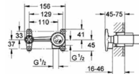
33 769 000 Wall mounted basin mixer set concealed body
