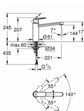
30 193 000 Sink mixer medium spout
