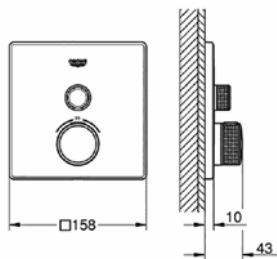
29 123 000 Grohtherm SmartControl thermostat for concealed installation with 1 valve
