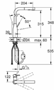
30 270 000 / 30 270 DC0 Sink mixer high spout with Pull-Out Dual Spray
