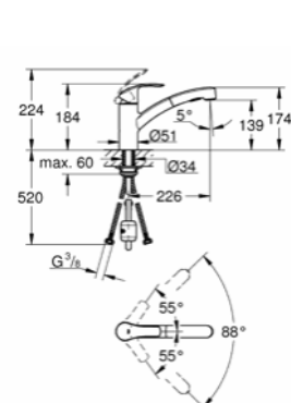
30 305 000 EuroSmart sink mixer with Pull-Out Spray
