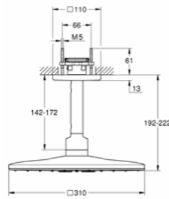
26 481 000 Rainshower 310 Head shower with wall arm
