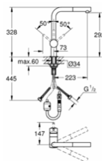
31 115 000 Sink mixer L-spout with Pull-Out Spray
