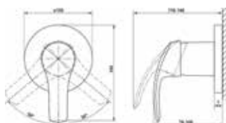
19 451 002SM + 33 962 000 Shower/bath mixer (Exclusive to ANZ)
