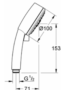
27 573 001 Hand shower 100
