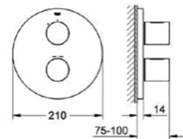
19 467 000 Grohtherm 3000 Cosmopolitan Thermostatic shower trim set
