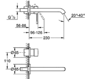
19 967 001 + 32 635 000 Wall mounted basin mixer set
