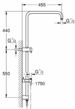
26 167 000 Twin shower system with diverter
