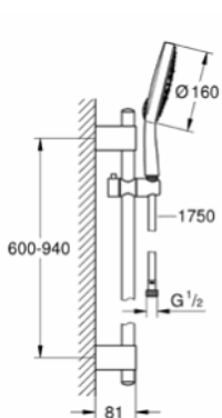
27 746 000 Power&Soul Cosmopolitan Rail shower 900mm Hand shower 160mm
