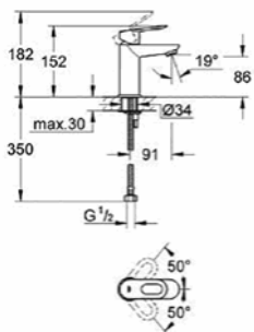
23 179 000 S-Size Basin mixer
