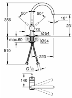
32 930 000 Sink mixer C-spout
