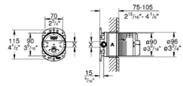
26 484 000 Rainshower® universal rough-in
