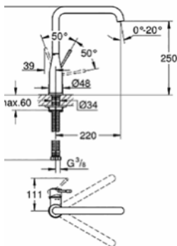
30 269 000 / 30 269 DC0 Sink mixer high spout
