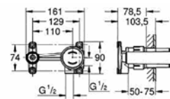
23 429 000 Wall mounted basin mixer set concealed body
