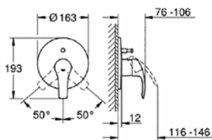
19 450 002 + 33 961 000 Shower/bath mixer with diverter
