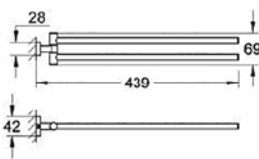
40 624 001 Double towel bar 439mm
