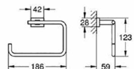
40 510 001 Towel ring
