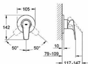
29 046 000 + 33 962 000 Shower/bath mixer
