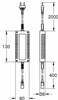
42 429 000 Power supply unit base box
