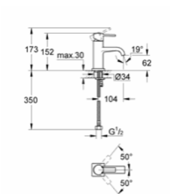
32 759 000 M-Size Basin mixer
