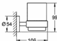
40 447 001 Glass tumbler holder
