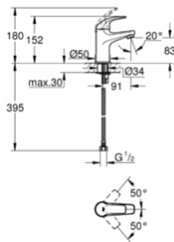
23 174 000 Basin mixer
