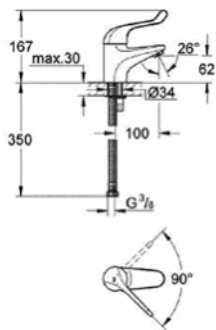
32 789 000 Euroeco Special Single-lever safety basin mixer 1/2"
