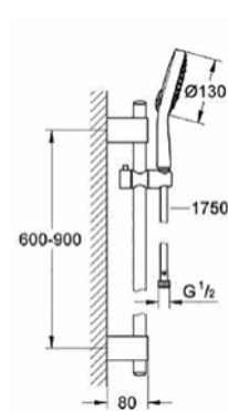
27 734 000 Power&Soul Cosmopolitan Rail shower 900mm Hand shower 130mm
