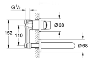
20 474 000 Wall mounted basin mixer set
