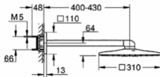
26 479 000 Rainshower 310 Head shower with wall arm
