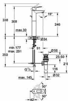
32 856 000 XL-Size Basin mixer for freestanding basins
