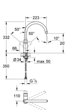
31 232 000 BauLoop Kitchen sink mixer
