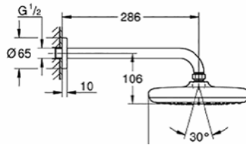
26 412 000 New Tempesta Cosmopolitan 210 Head shower with wall arm
