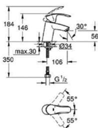
33 161 002 Basin mixer
