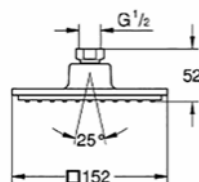
27 705 000 Euphoria Cube 150 Head shower 152 x 152mm
