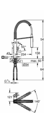
31 395 000 Professional sink mixer with Professional Spray
